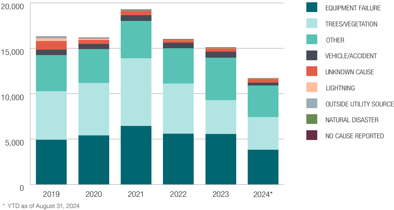
Figure A-2: System-wide transmission outages and cause, by year
